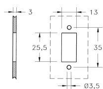
Forma standard / Standard form
