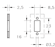
Forma mignon / Mignon form
